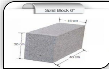
Concrete Blocks
